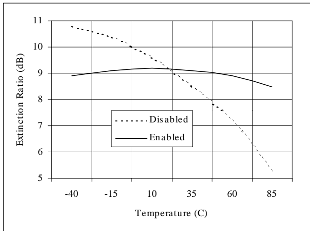
Figure 4. Measured extinction ratio vs. temperature with compensation disabled and enabled
